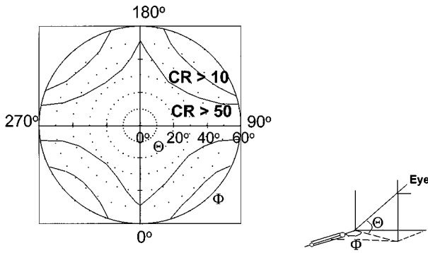
FIG. 5. Iso-contrast plot of an HTP cell. The contrast ratio CR is defined as the ratio of the intensity of the transmitted light in the on state to that of the off state at 30 V.
