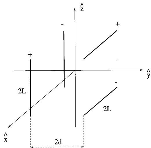
FIG. 1. Schematic diagram of the HTP mode electrode configuration.
