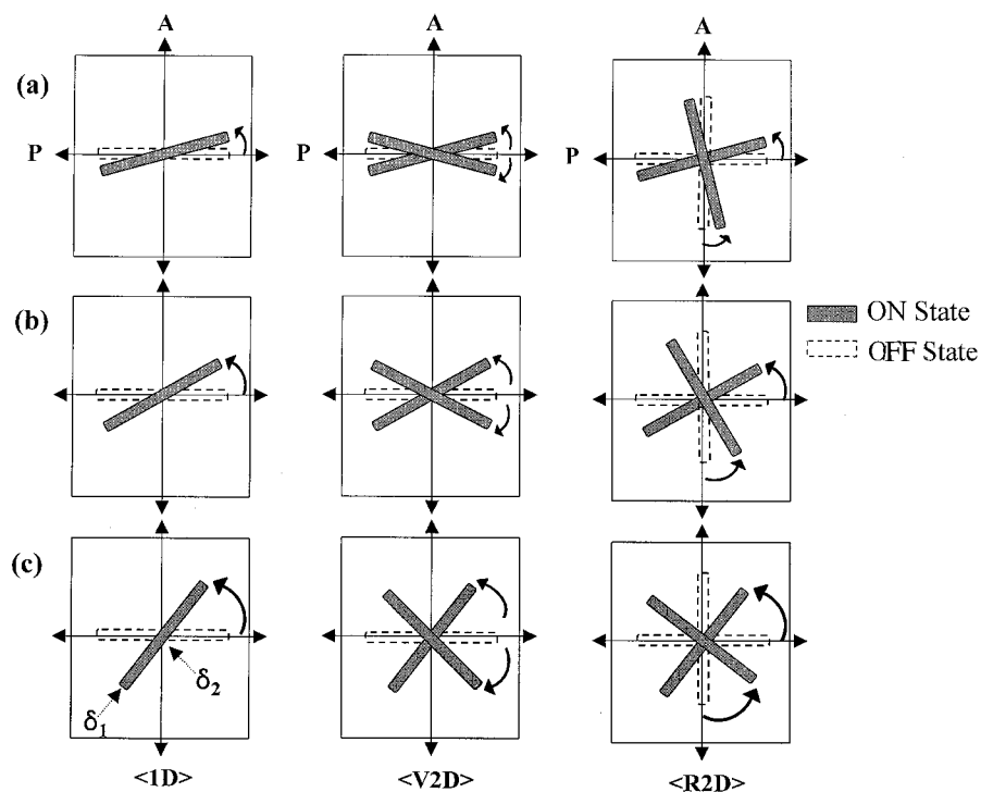
Figure 3. Configuration of the LC director in the IPS devices with 1-D, V2-D and R2-D structures at (a) V_{10} , (b) V_{50} and (c) V_{100} .
