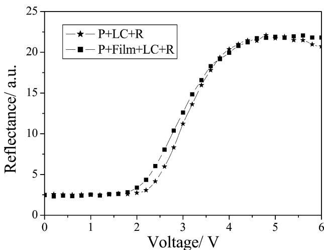
Figure 8. Measured voltage-dependent reflectance.
