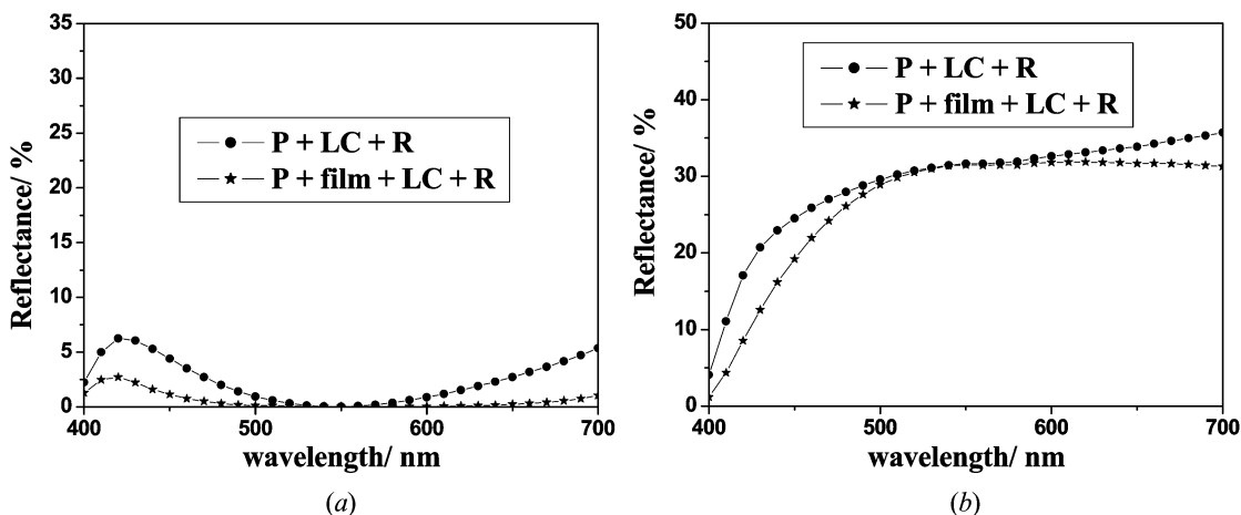
Figure 4. Wavelength dependence of (a) dark state and (b) white state, in reflectance.
