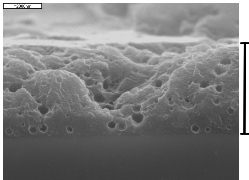
Figure 5. SEM image for the NT PDLC cell made under LC 70 wt%, curing temperature of 20 ^{\circ}\text{C} , and strong UV intensity of 198 mW/cm 2 .
