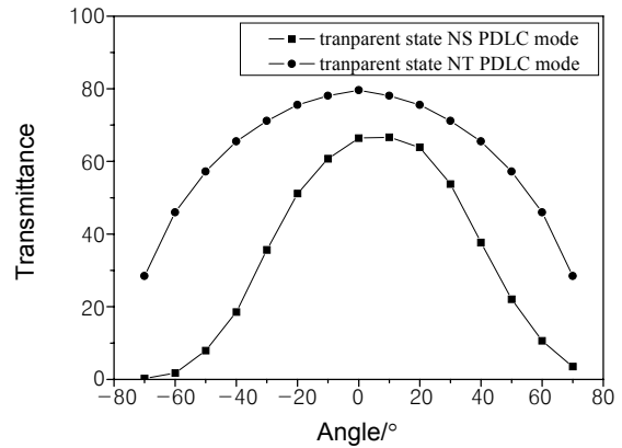
Figure 6. Comparison of viewing angle characteristics in transparent state between the NT PDLC cell with LC 70 wt%, curing temperature, 20 ^{\circ}\text{C} and strong UV intensity, 198 mW/cm 2 and the conventional NS PDLC cell.
