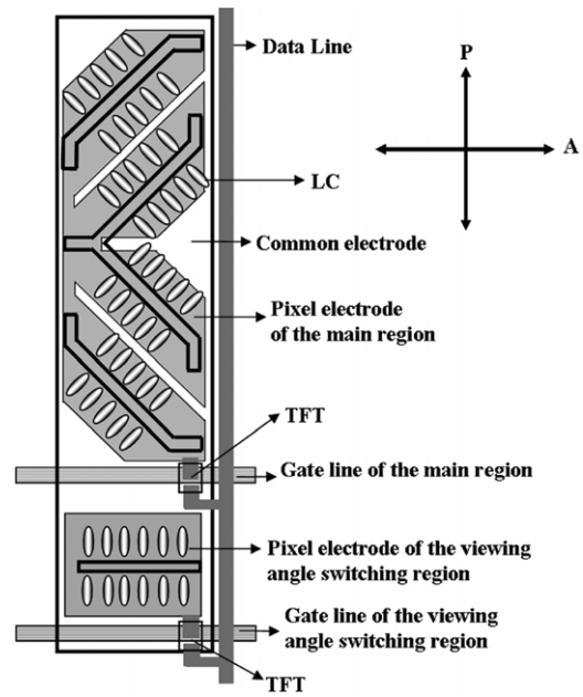
Figure 2. Electrode structure of the controllable viewing angle PVA-LCD with LC director direction in the on state.
