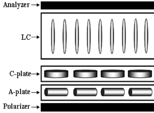
Figure 1. Schematic configuration of the film compensated VA device.
