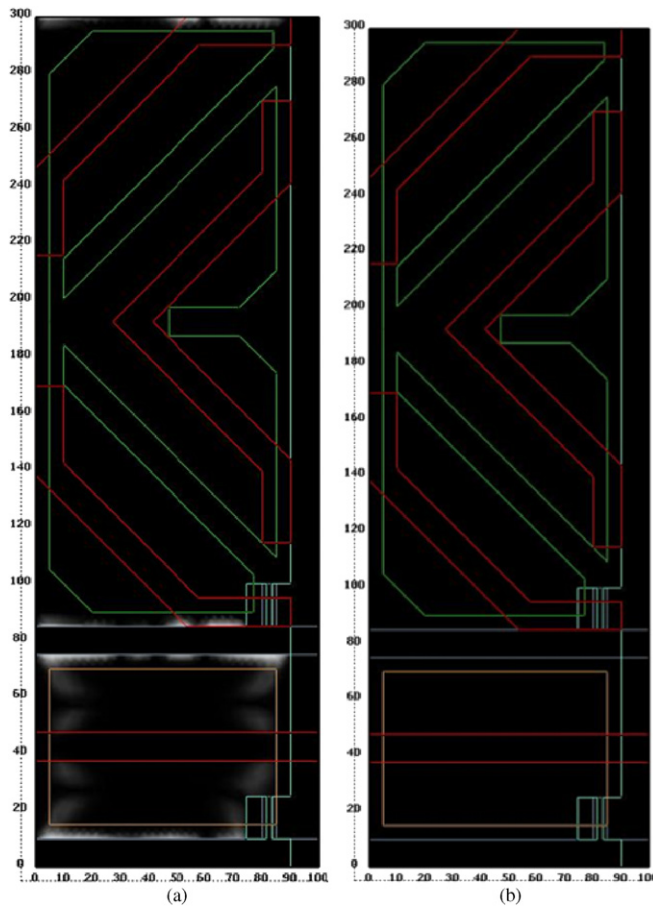
Figure 4. Light leakage of the controllable viewing angle PVA-LCD in the dark state: (a) narrow and (b) wide viewing angle modes.
