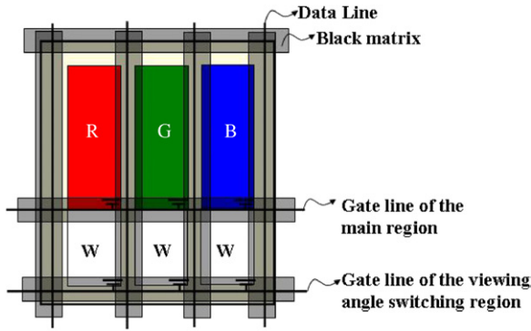
Figure 3. Arrangement of colour filter corresponding to figure 2. (This figure is in colour only in the electronic version)
