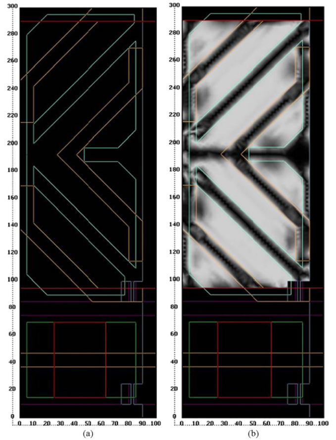
Figure 5. (a) Dark and (b) white states of the controllable viewing angle PVA-LCD using BM for both narrow and wide viewing angle modes.
