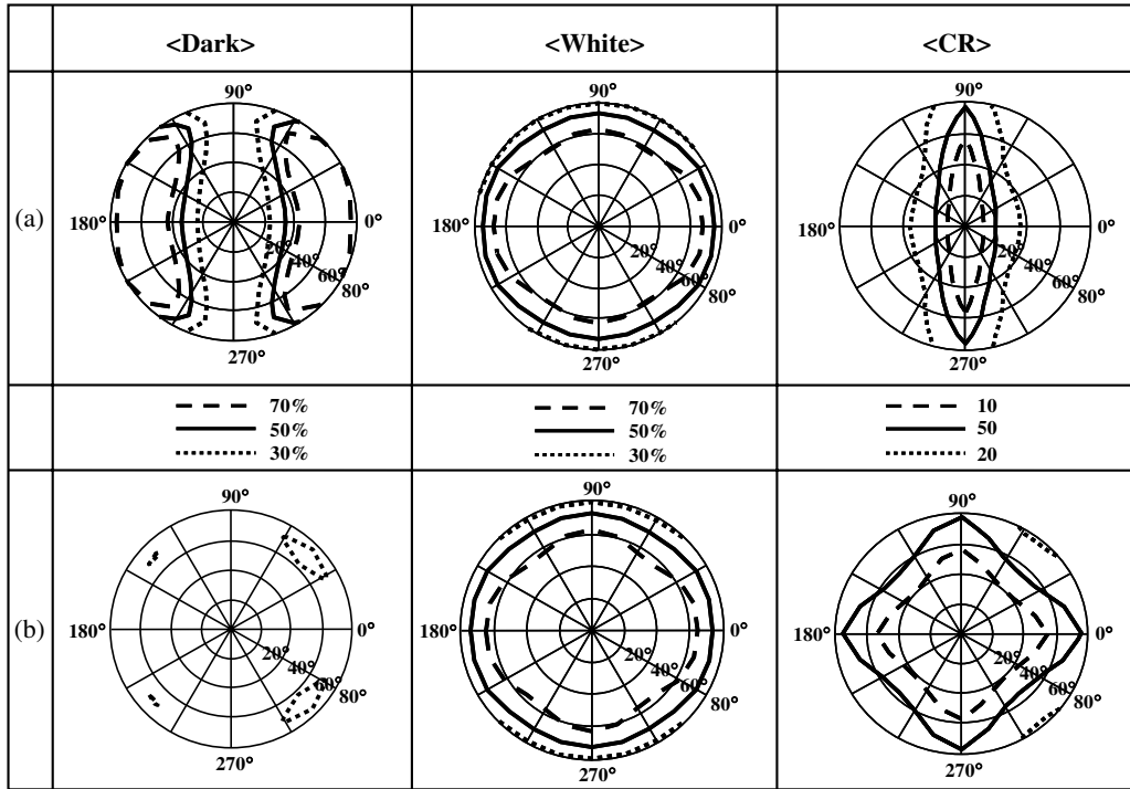
Figure 6. Iso-transmittance curves in the white and dark states and iso-contrast curves: (a) narrow viewing angle mode and (b) wide viewing angle mode.
