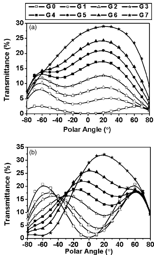
FIG. 3. Simulated viewing-angle dependences of eight gray levels as a function of polar angle along the horizontal direction: (a) WVA mode and (b) NVA mode.
