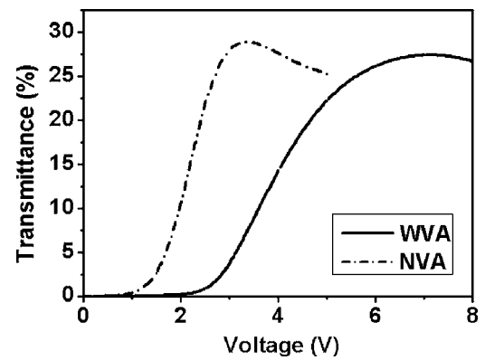
FIG. 2. Voltage-dependent transmittance curves in the proposed viewing-angle switching display when the incident light is 550 nm.
