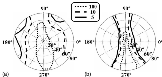
FIG. 4. Isocontrast curves at an incident wavelength of 380–780 nm: (a) WVA mode and (b) NVA mode.
