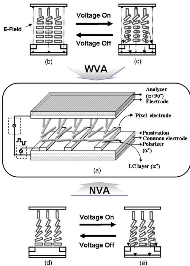
FIG. 1. (Color online) Schematic configuration of a proposed viewing-angle controllable display with LC orientation and driving scheme: (a) fringe- and vertical-field driven cell structures, (b) dark and (c) white states in the WVA mode, and (d) dark and (e) white states in the NVA mode.
