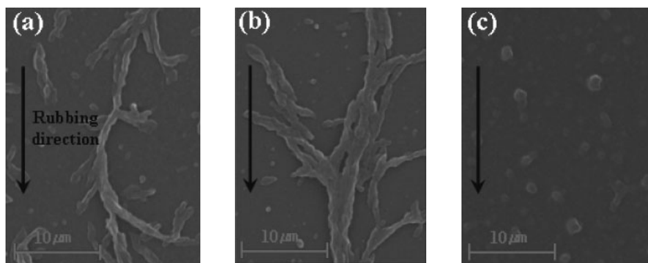
Fig. 10. SEM images of the inside surface of ECB-VA cell prepared at different curing intensities: (a) 246.3 \text{ mW/cm}^2 \times 30 \text{ min} , (b) 98.5 \text{ mW/cm}^2 \times 74 \text{ min} , and (c) 5.0 \text{ mW/cm}^2 \times 24 \text{ h} .
