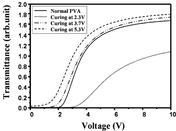
Fig. 5. Voltage-transmittance curves according to various curing voltages when the weight percent of RM monomer is fixed at 0.1%.
