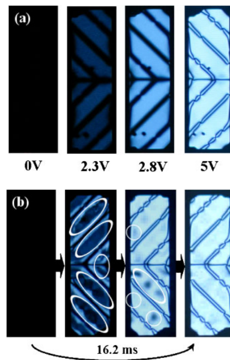
Fig. 3. (Color online) (a) Micro LC textures of the normal PVA cell as a function of applied voltages and (b) time-resolved LC textures with applied voltage of 5 V.
