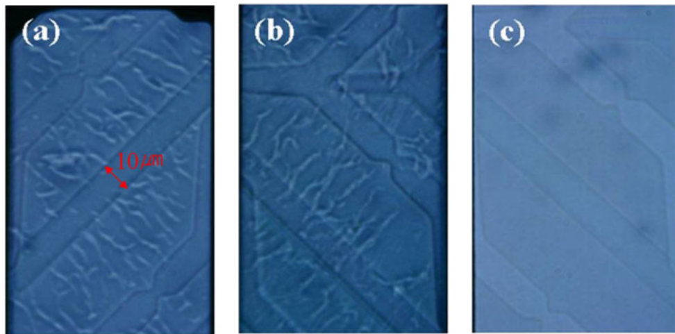
Fig. 9. (Color online) POM images of the inside surface of PVA cell prepared at different curing intensities: (a) 246.3 \text{ mW/cm}^2 \times 30 \text{ min} , (b) 98.5 \text{ mW/cm}^2 \times 74 \text{ min} , and (c) 5.0 \text{ mW/cm}^2 \times 24 \text{ h} .
