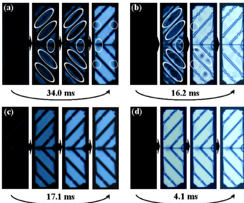
Fig. 6. (Color online) Time-resolved LC textures for comparison of LC dynamics responding to the applied voltages to reach T_{50} and T_{90} of maximal transmittance: (a) and (b) in the normal PVA cell and (c) and (d) in the surface-modified PVA cell cured at 3.7 V when the weight percent of RM monomer is 0.1%, respectively.
