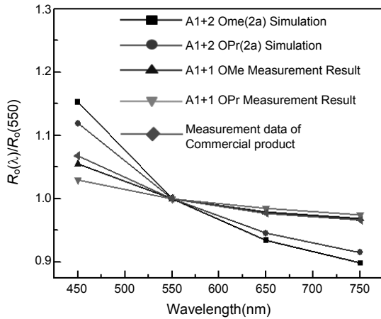
Figure 9. Comparison of R_0 wavelength dispersion between simulated and experimental results in the case of A1 with methoxy and propionate groups.
