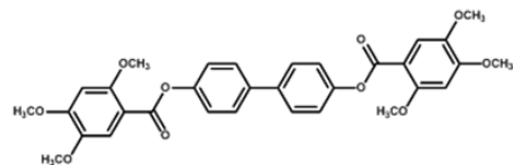
Figure 3. Selected molecular structure with biphenyl core fragment.
