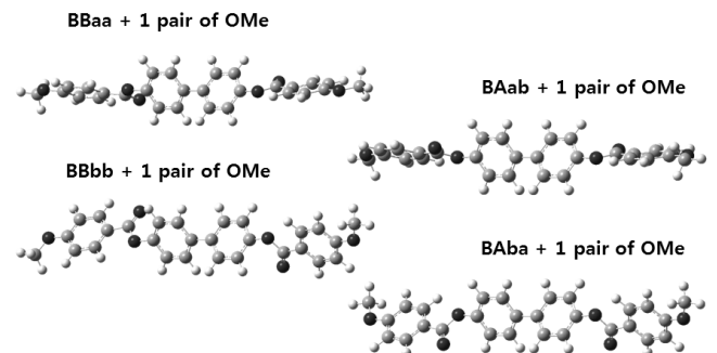
Figure 4. A1 isomer structure that was substituted with one pair of methoxy group: red ball-carbonyl group.
