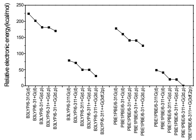
Figure 2. Relative energy according to basis function.
