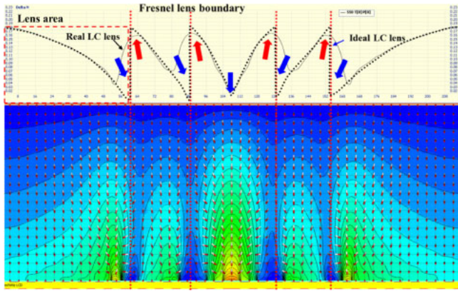
Fig. 2. (Color online) Simulation result of refractive index distribution of Fresnel LC lens (dotted line) compared with ideal Fresnel lens (solid line) with LC director profile and the electric potential energy distribution in MeD Fresnel LC lens. The profile of proposed lens does not match ideal lens. The rectangular area with dotted line and vertical dotted lines indicate domains for lens and lens boundary, respectively.
