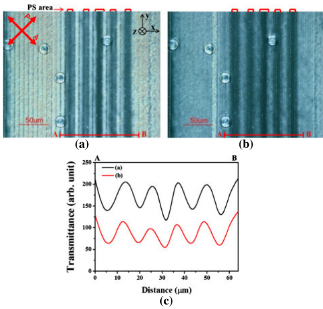
Fig. 4. (Color online) Observed polarizing optical microscope image after polymer stabilization of surface pretilt angle at the lens boundary: (a) 0 V and (b) 10 V. The light intensity across the x -axis of the microscope images along the line AB also confirms the existence of pretilt angle locally (c). Here P and A indicate polarizer and analyzer, respectively and five circles in the images are plastic ball spacers to keep the cell gap.
