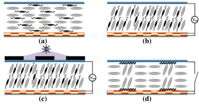
Fig. 3. (Color online) Schematic drawings of controlling pretilt angle locally via polymer stabilization process: (a) the mixture is homogeneously aligned, (b) the vertical field is applied to the cell, (c) the UV is exposed to the lens boundary via UV mask, and (d) high surface tilt angle is formed at the lens boundary even after the voltage is released.
