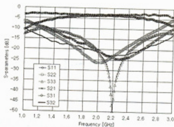
(b) 소형화된 발룬 (b) Balun with size-reduction
