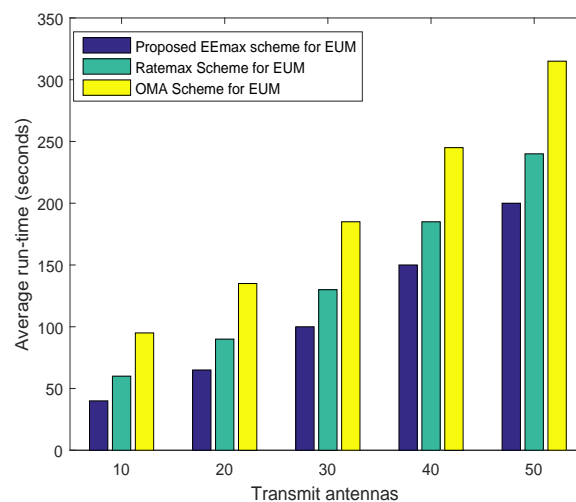
Figure 4. Average run-time versus number of transmit antennas.
