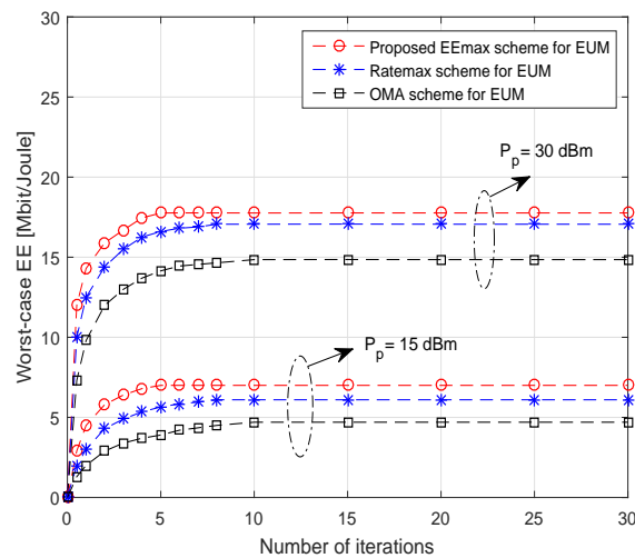
Figure 3. Worst-case EE versus number of iterations.
