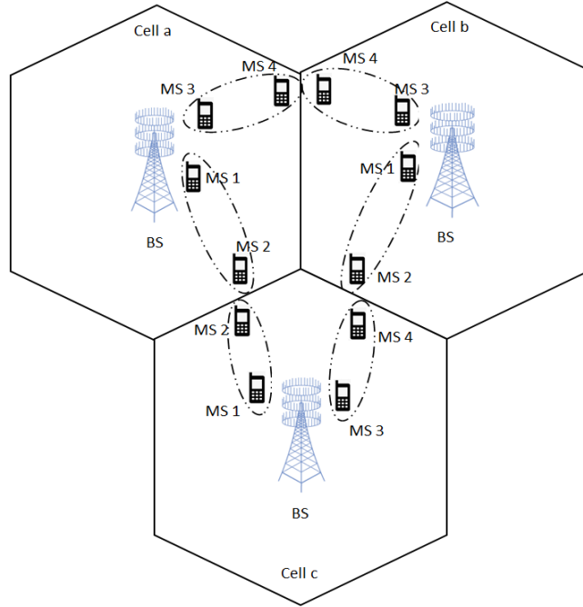
Figure 1. Multicell Massive multiple-input multiple-output non-orthogonal multiple access (MIMO-NOMA) downlink system.
