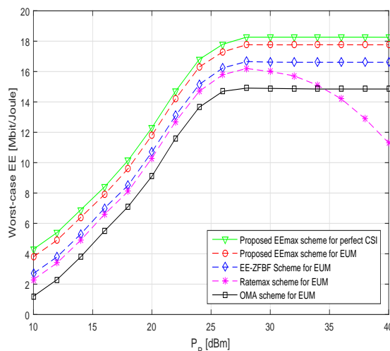
Figure 2. Worst-case energy efficiency (EE) versus transmission power P_p .
