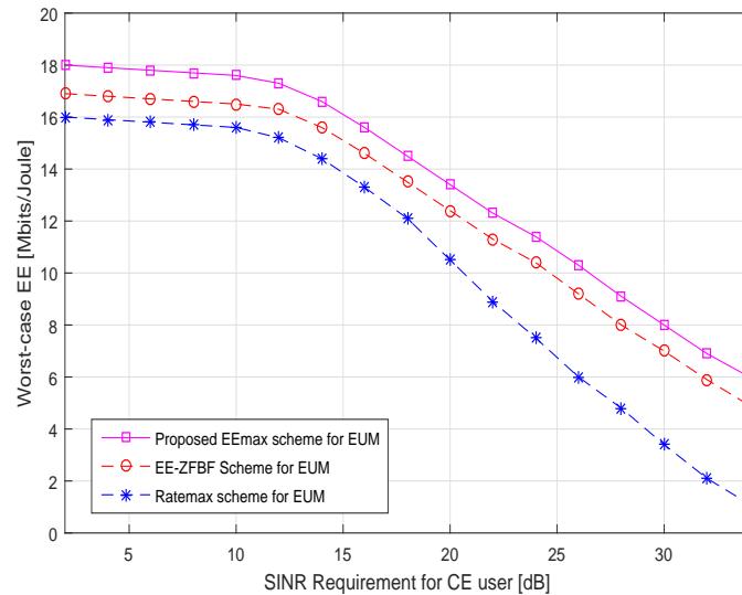
Figure 5. Worst-case EE versus signal-to-interference-plus-noise-power-ratio (SINR) requirement for cell edge (CE) users.
