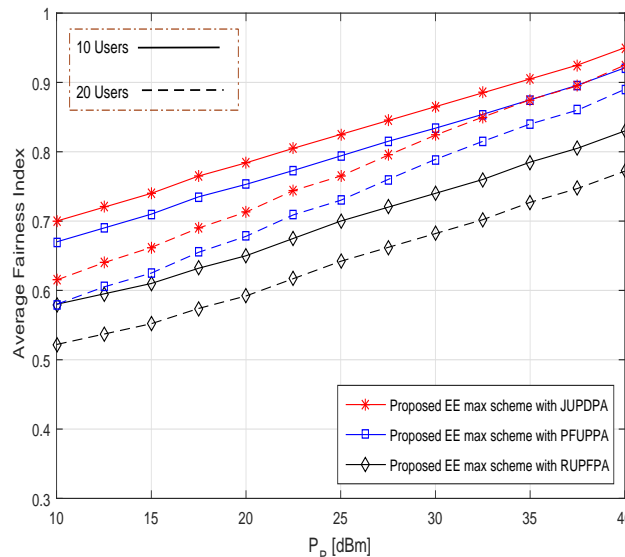
Figure 6. Average Fairness Index versus transmission power P_p .
