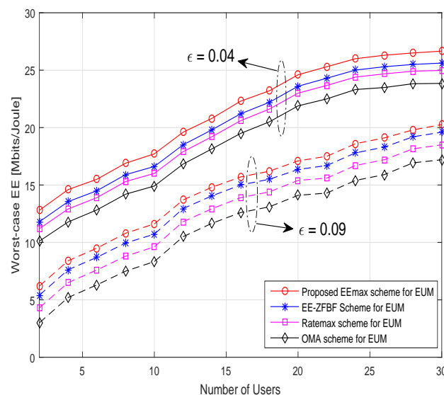
Figure 7. Worst-case EE versus number of users.
